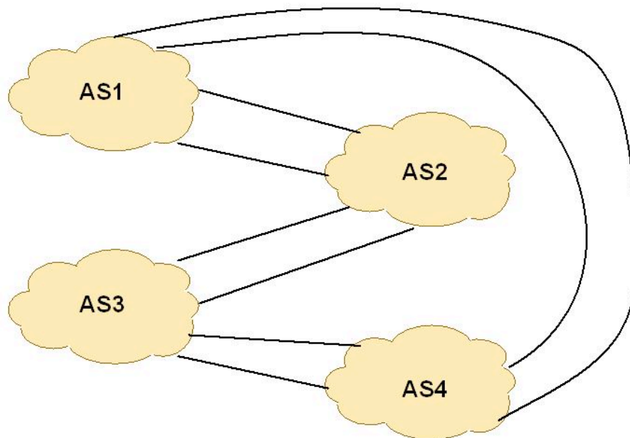
Figure 2 – AS relationship
